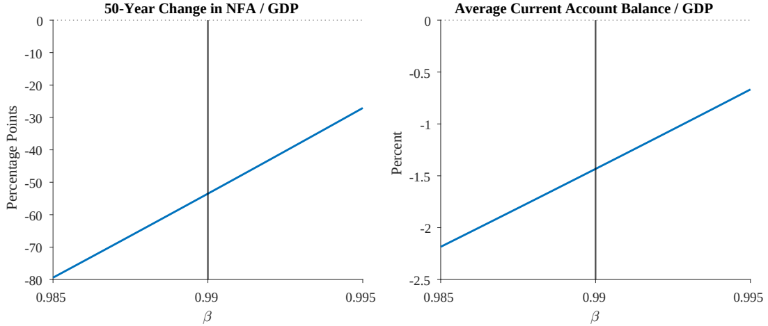
Figure 5: Sensitivity to the Discount Factor
