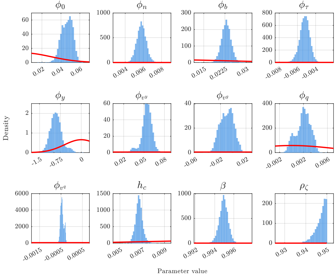
Figure 12: Priors and posteriors of the parameters of the consumption function
