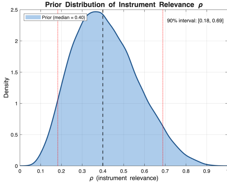
Figure 11: Prior distribution of instrument relevance. Instrument relevance is defined as \rho_i = M_i^2 / (M_i^2 + \sigma_{\eta,i}^2) , where M_i is the loading of instrument i on its assigned structural shock and \sigma_{\eta,i}^2 is the measurement-error variance. The figure is simulated from the priors M_i \sim \text{Gamma}(20, 0.025) and \sigma_{\eta,i}^2 \sim \text{Gamma}(4, 0.1) .
