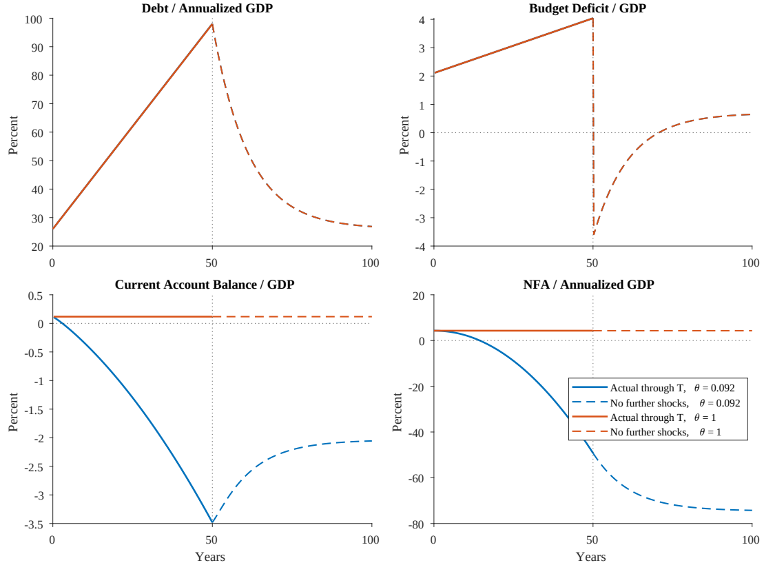
Figure 2: A Fifty-Year Increase in Government Debt
