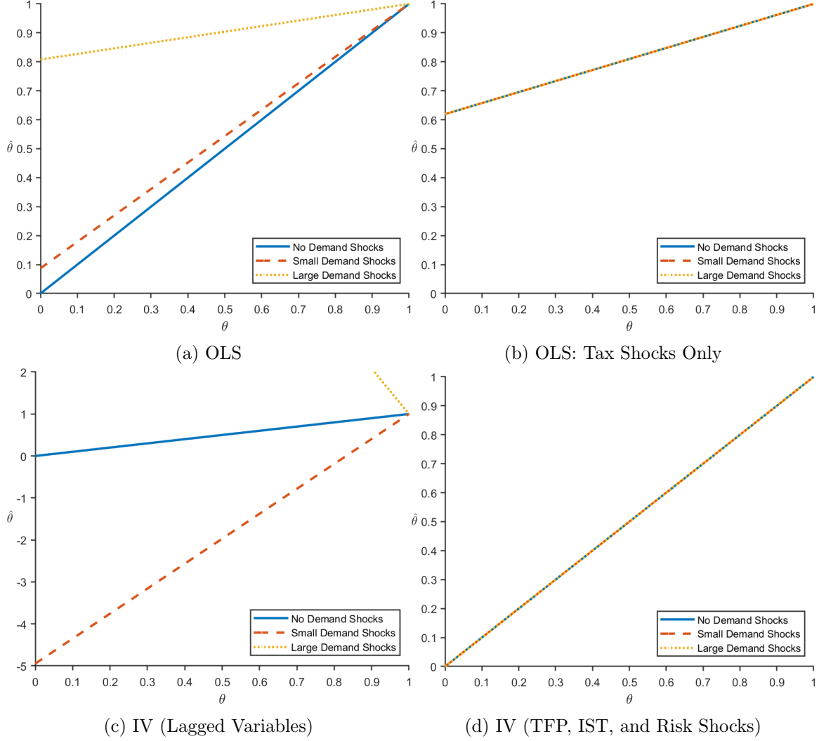
Figure 4: Population Regression Coefficients for the Consumption Function
