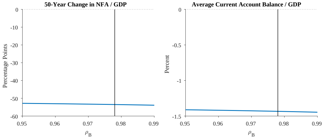
Figure 7: Sensitivity to Debt Persistence
