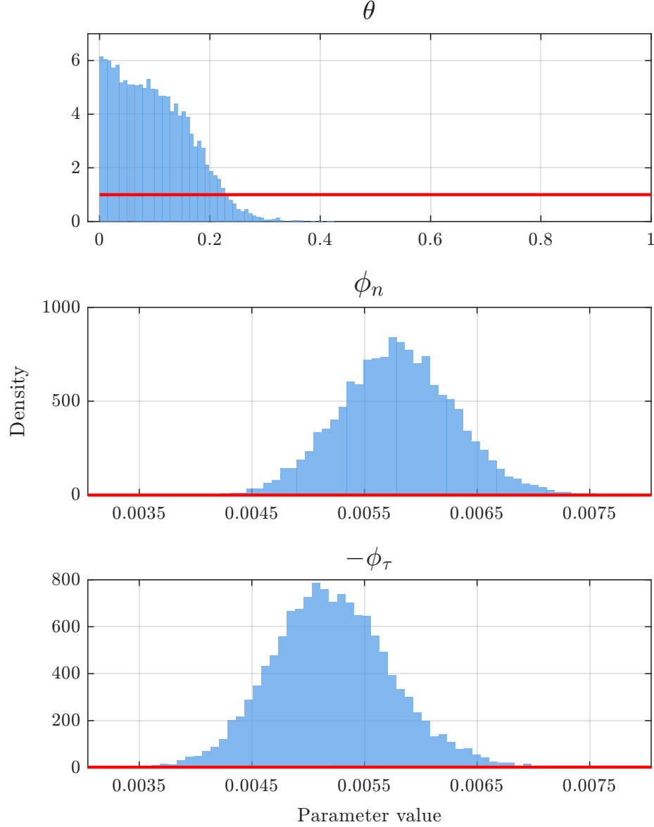
Figure 1: Marginal Posterior Densities for Three Consumption Function Parameters
