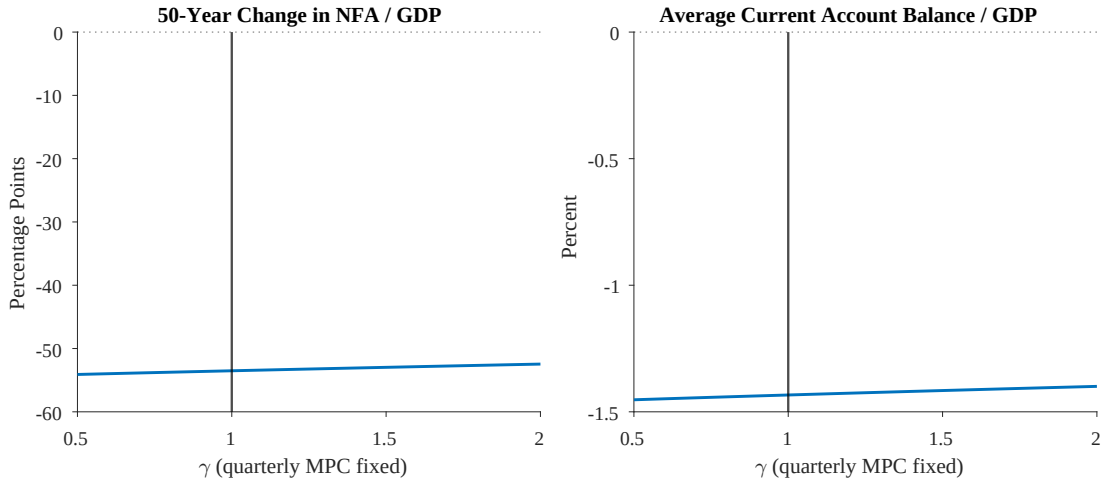
Figure 6: Sensitivity to Risk Aversion at a Fixed MPC
